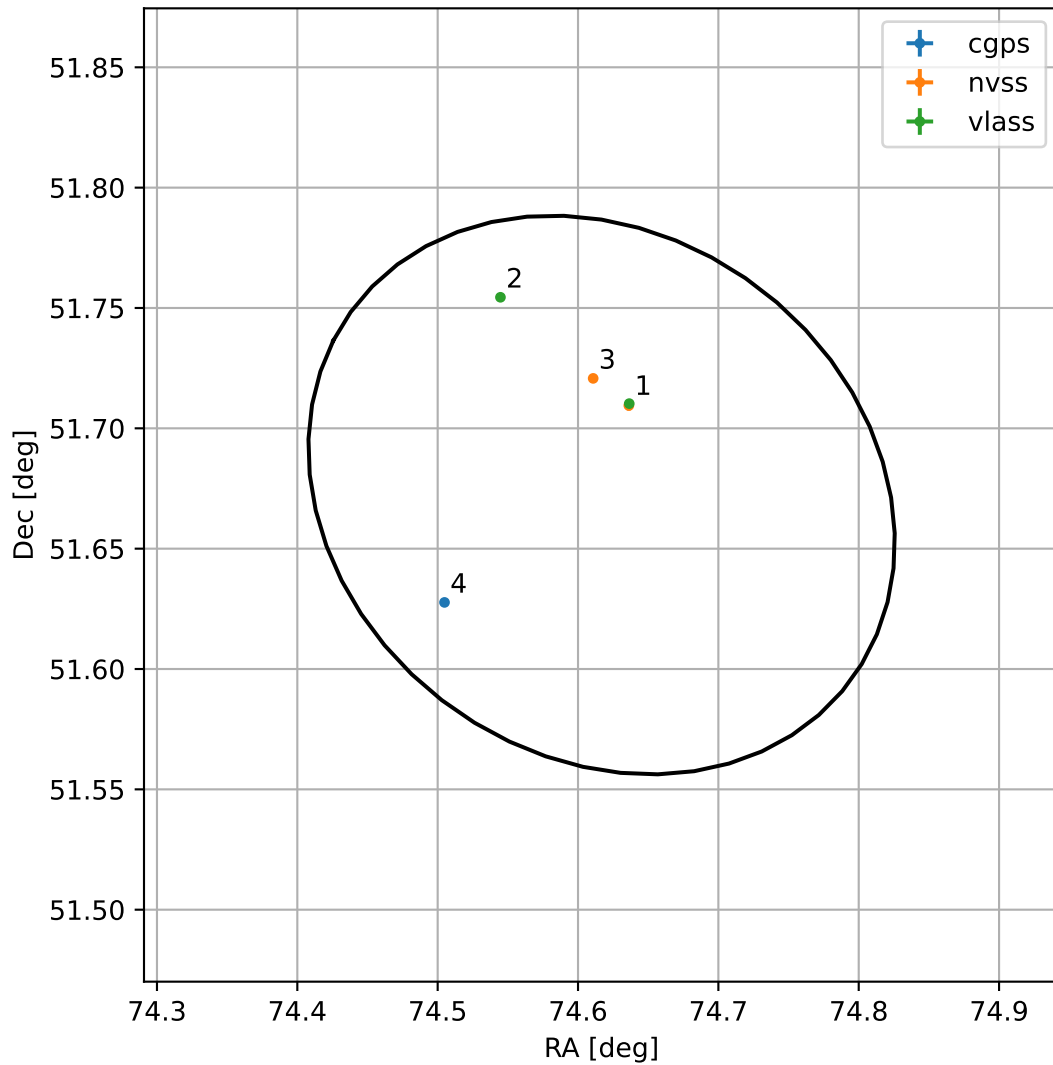
4FGL J0458.4+5140
