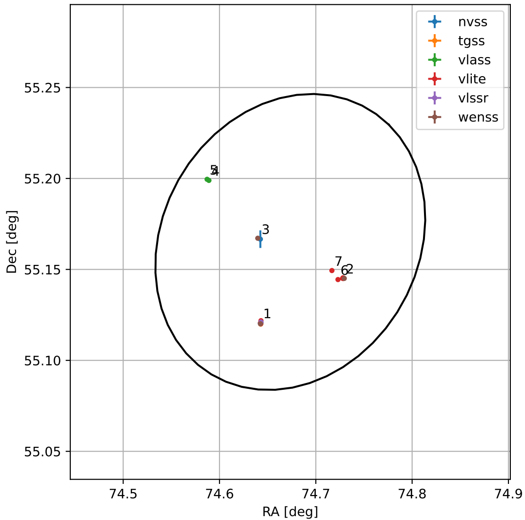
4FGL J0458.6+5509
