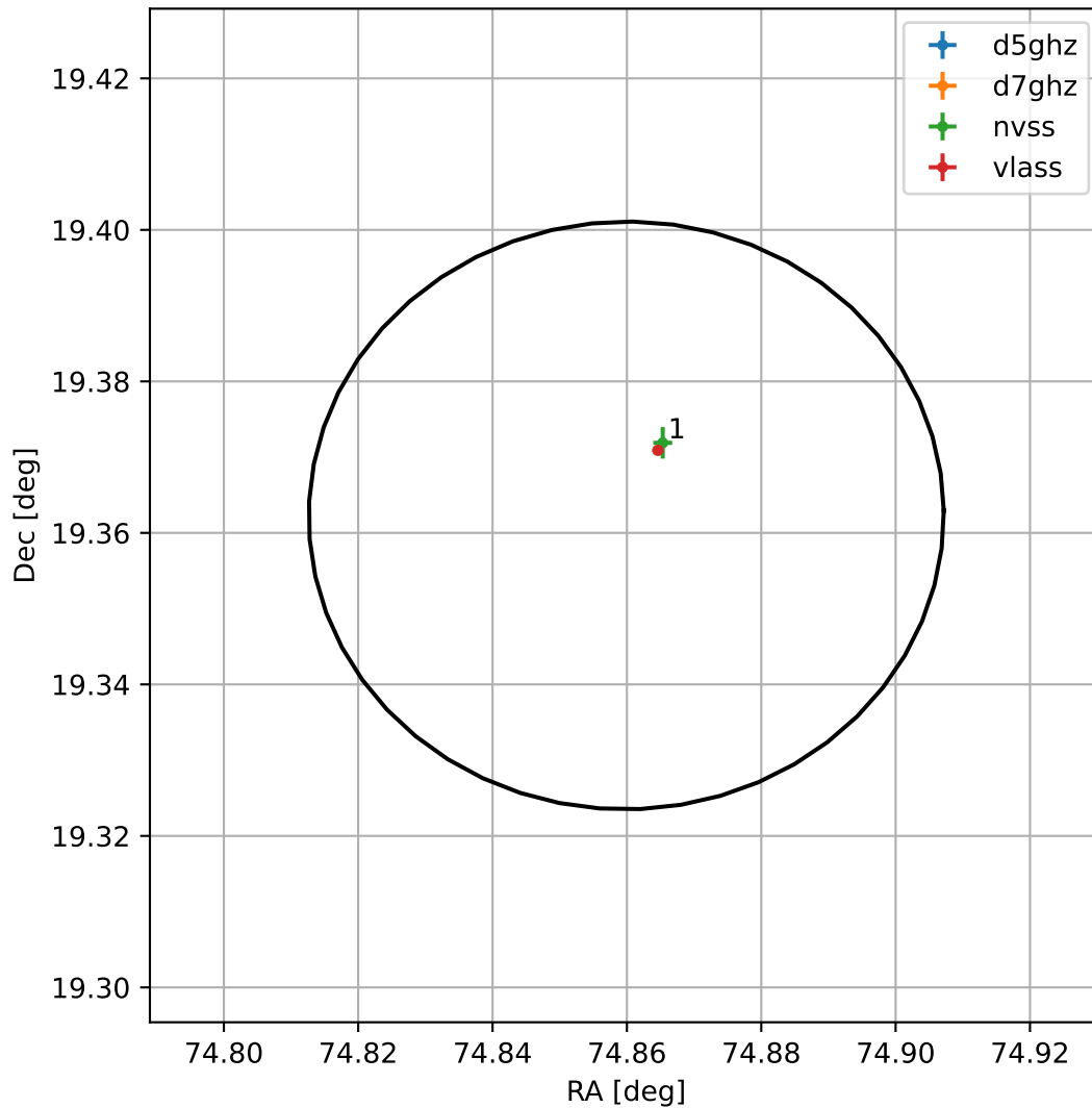
4FGL J0459.4+1921
