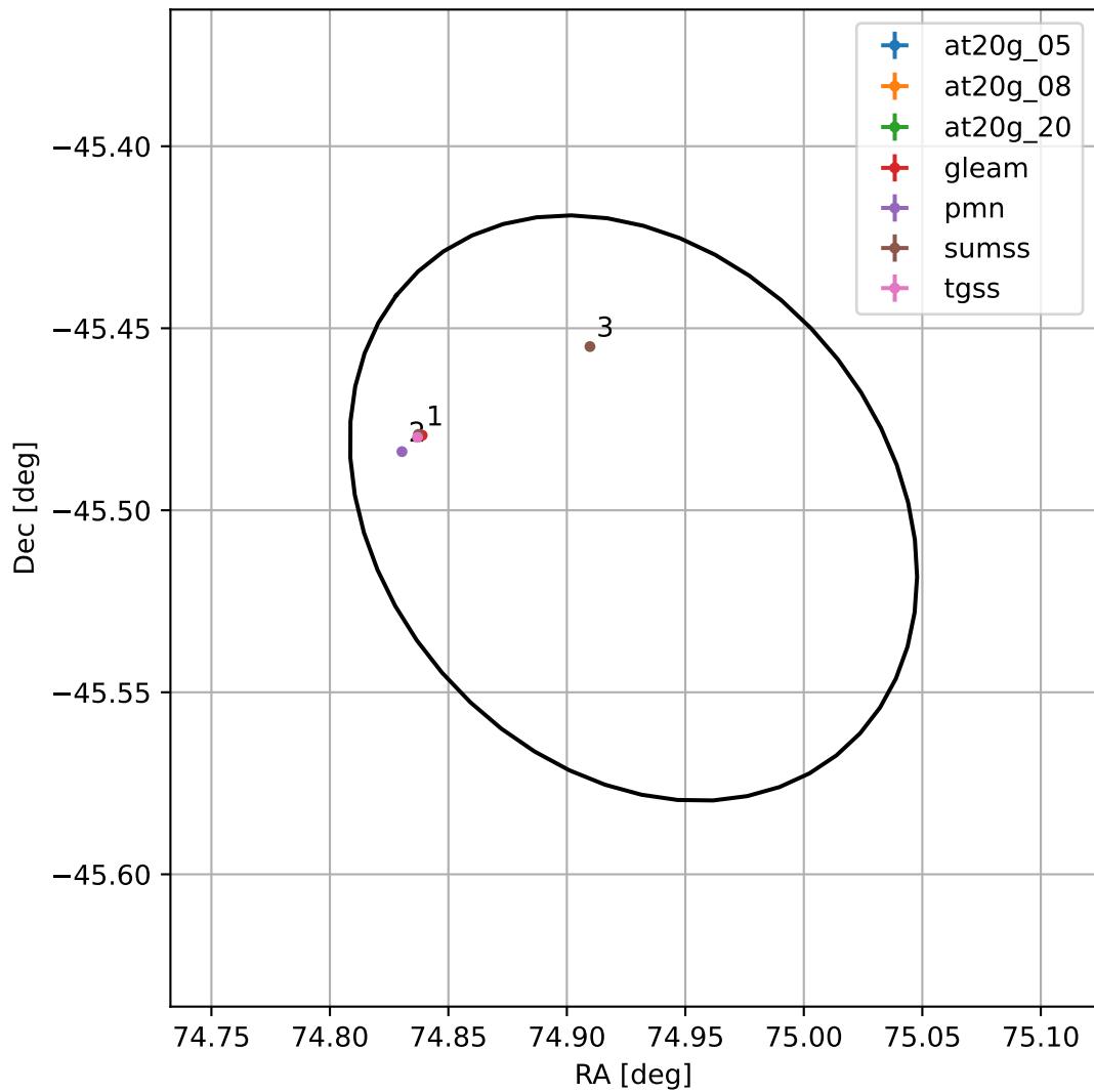
4FGL J0459.7-4529
