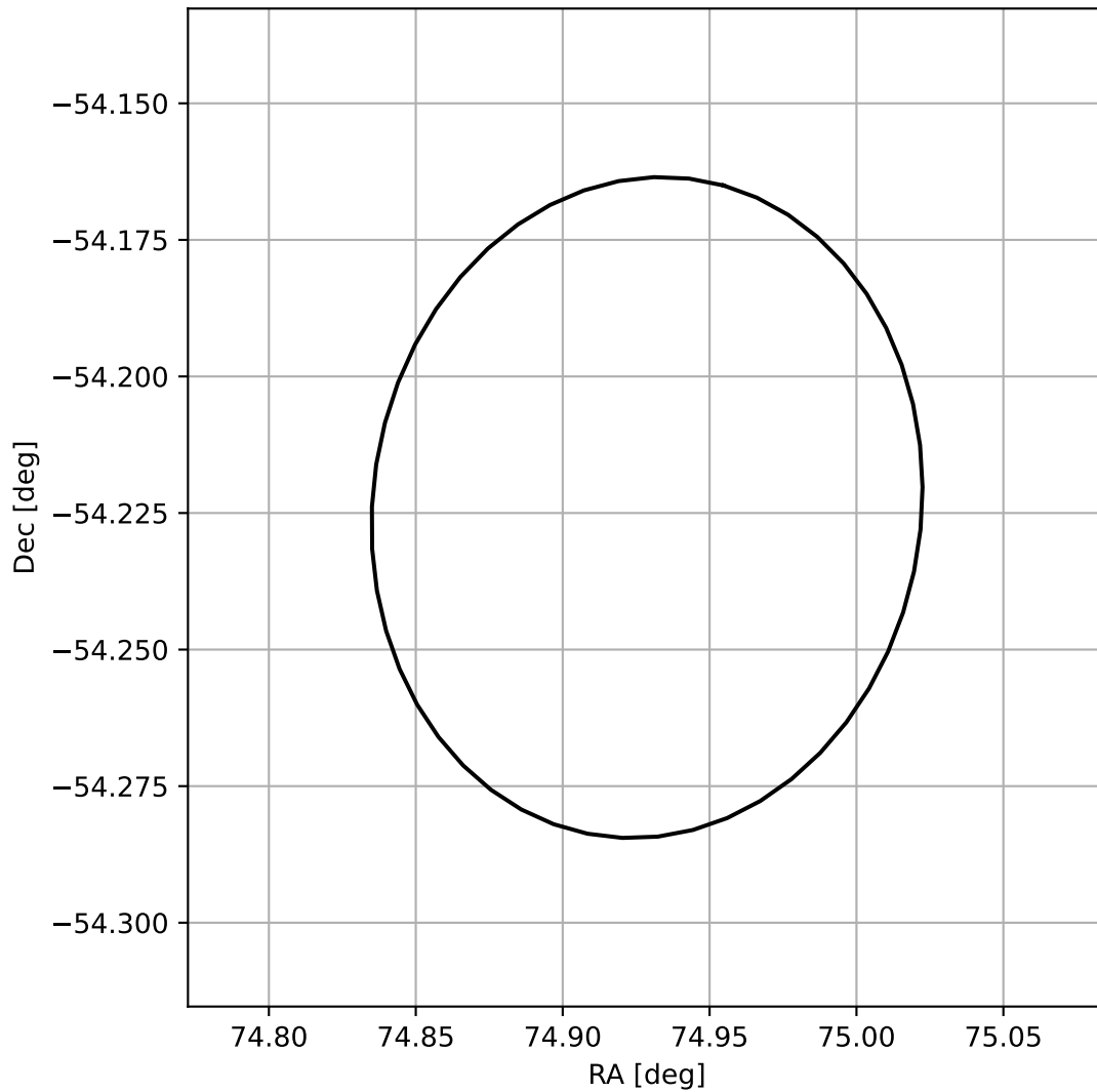
4FGL J0459.7-5413
