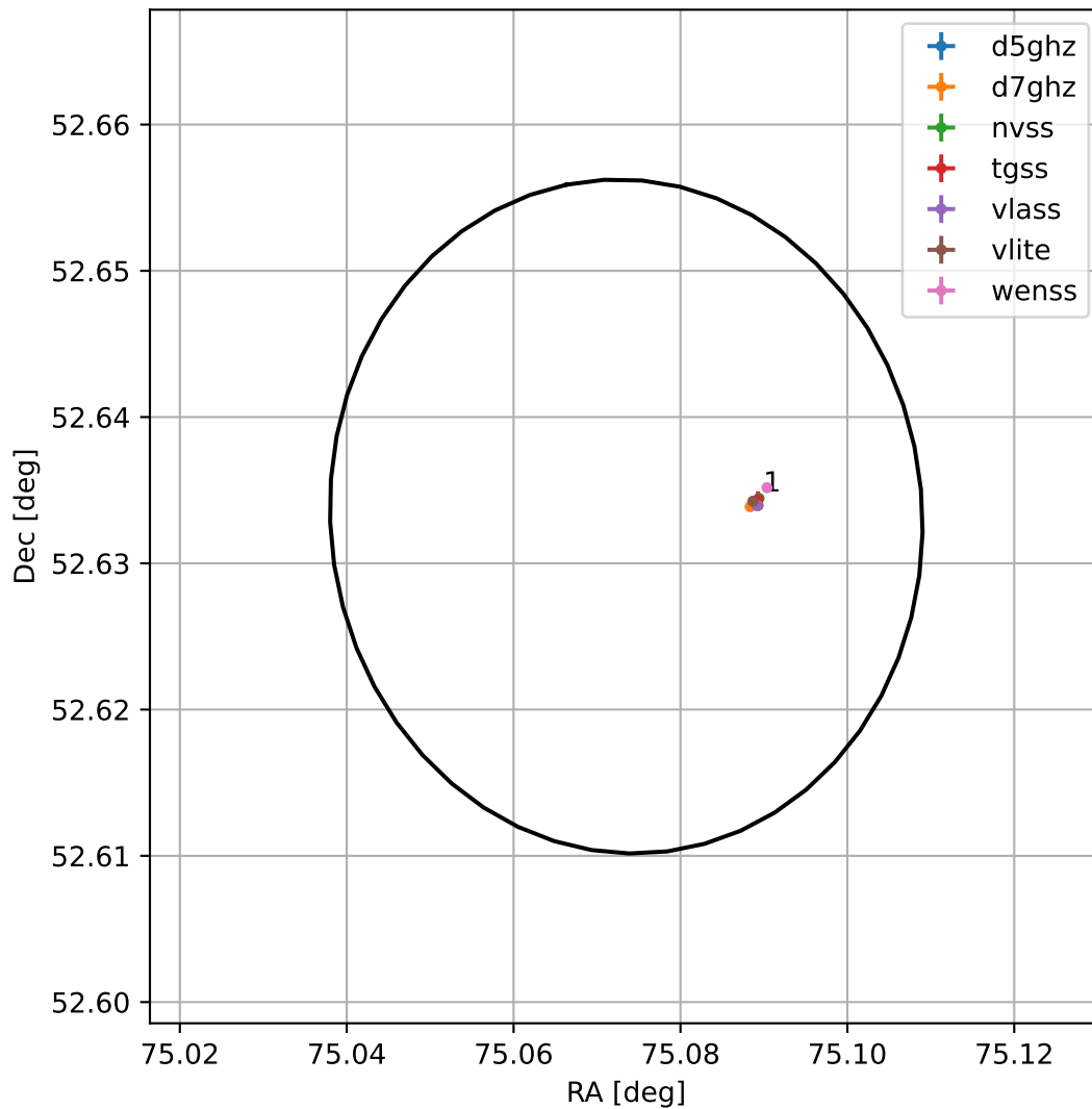
4FGL J0500.2+5237
