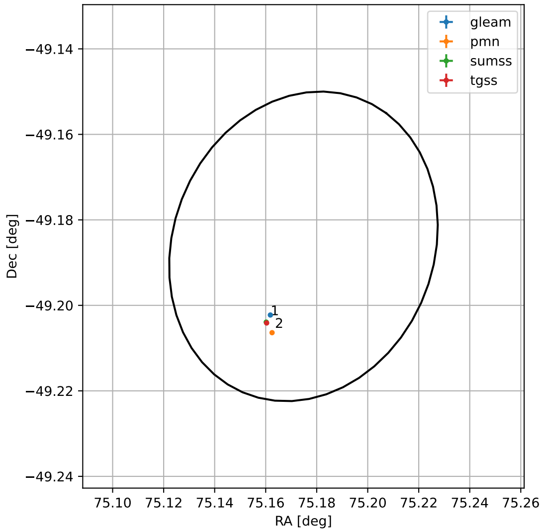
4FGL J0500.6-4911
