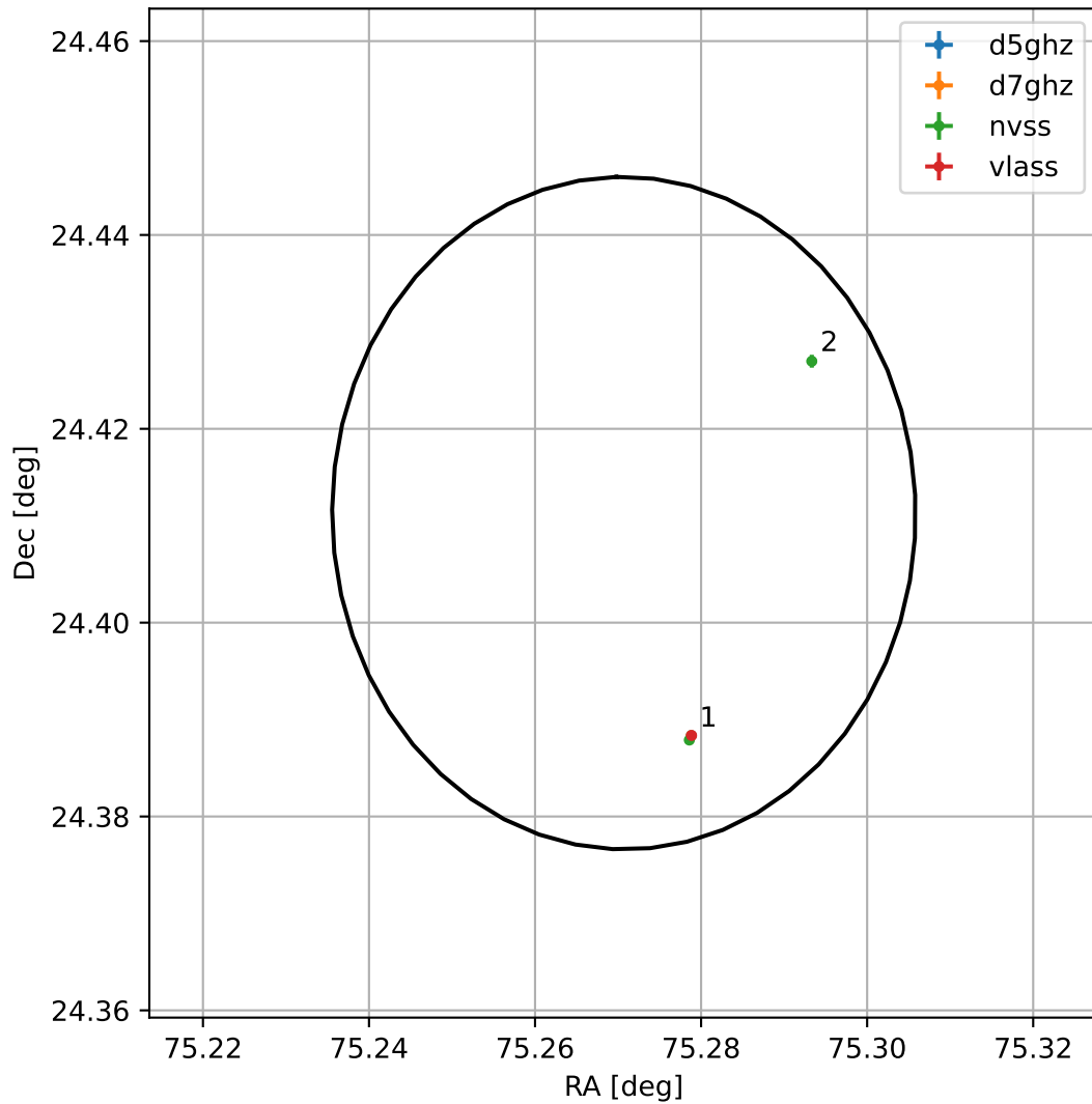
4FGL J0501.0+2424
