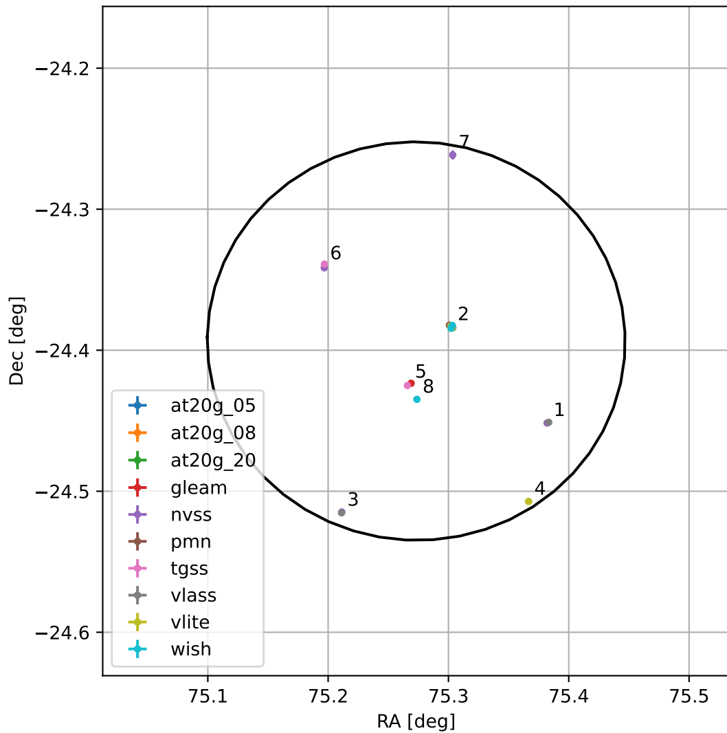
4FGL J0501.0-2423
