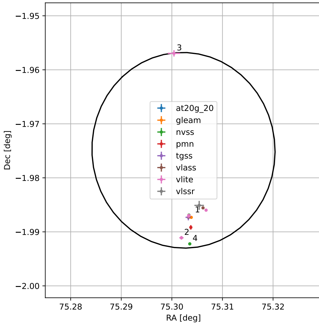
4FGL J0501.2-0158
