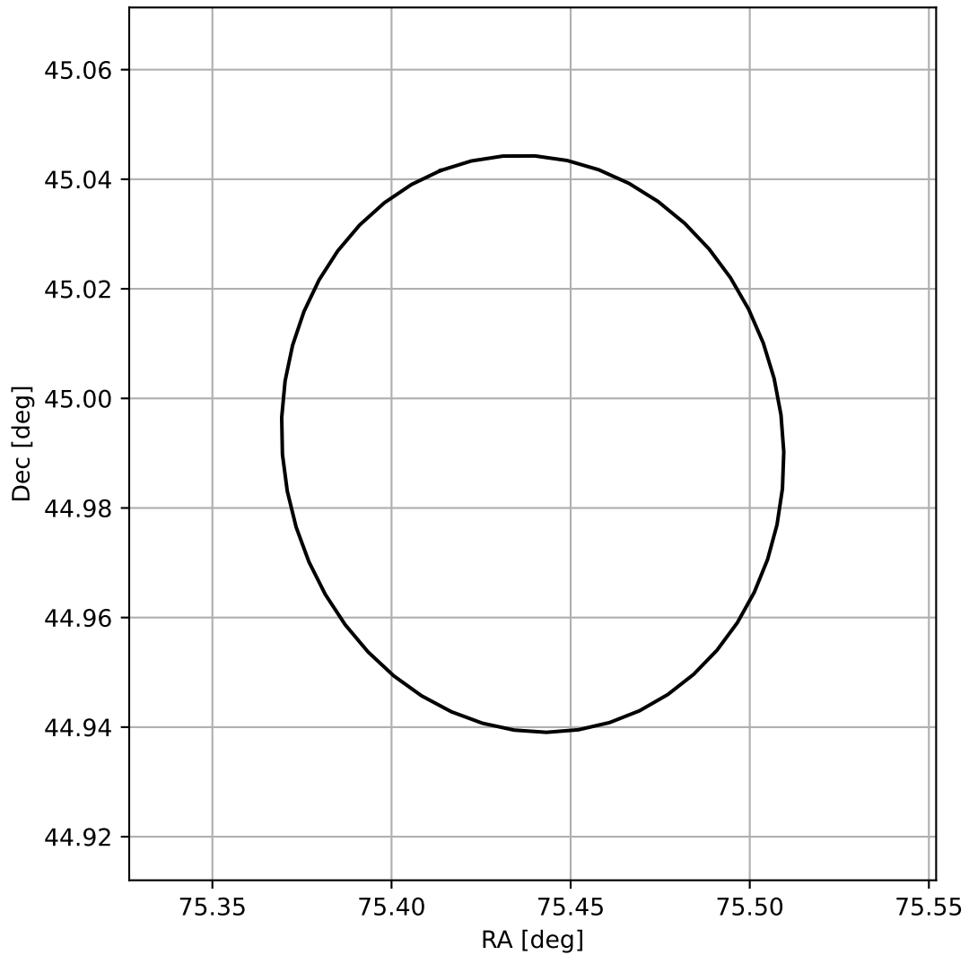
4FGL J0501.7+4459
