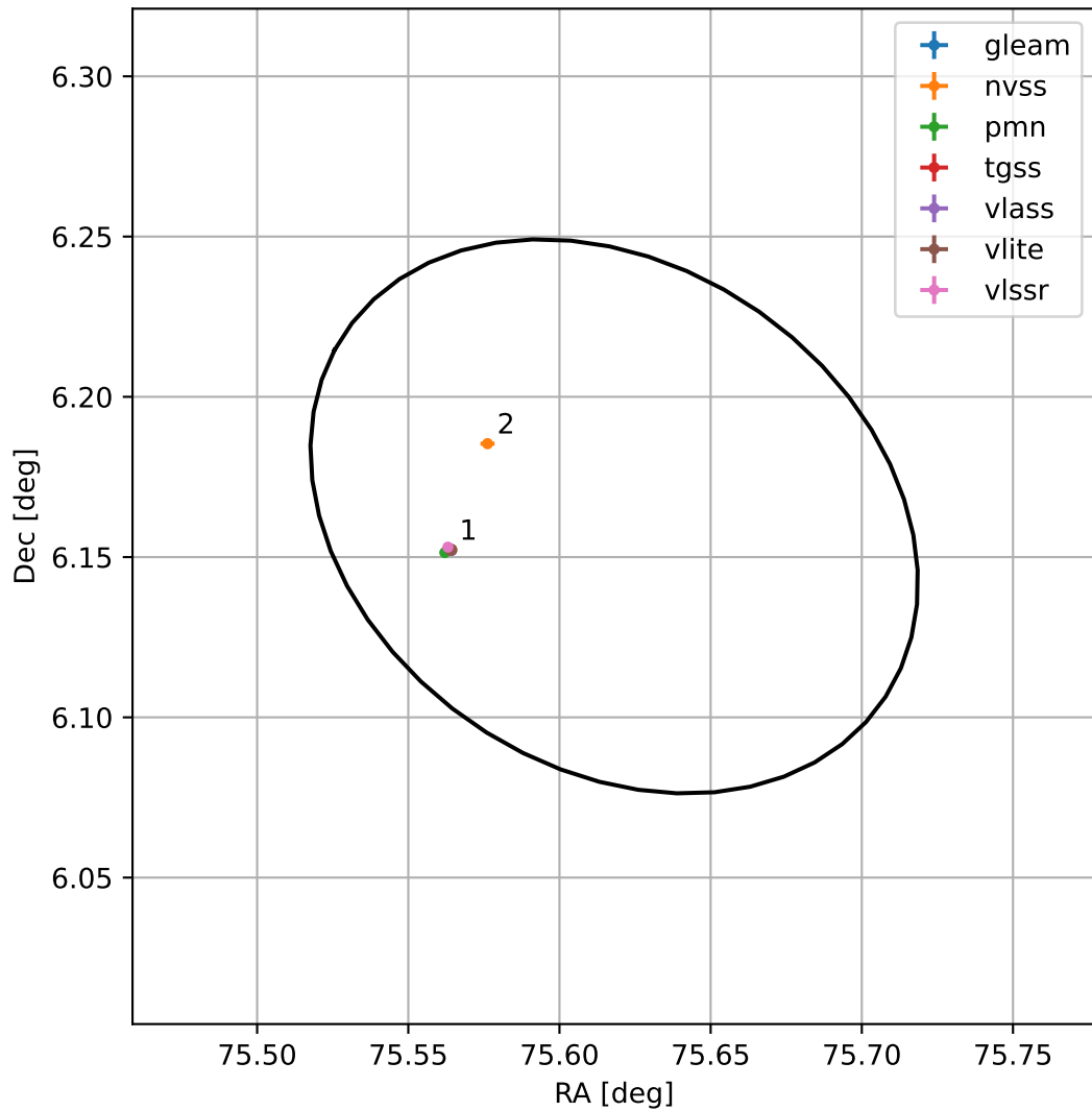
4FGL J0502.4+0609
