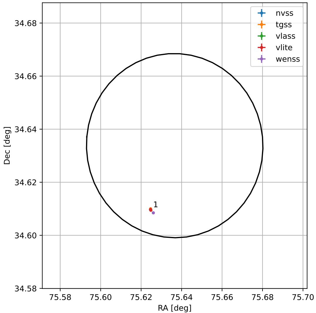
4FGL J0502.5+3438
