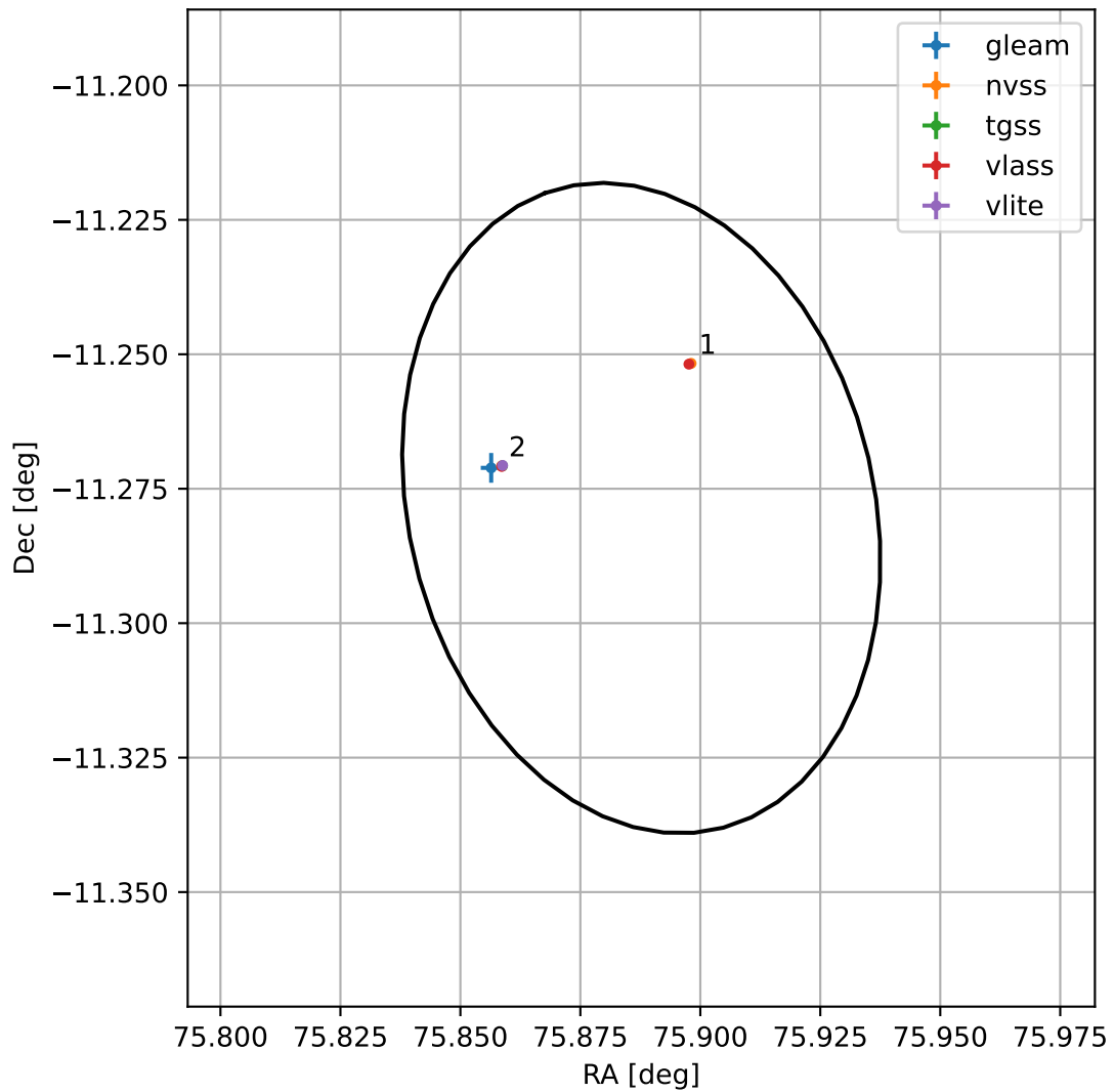
4FGL J0503.5-1116
