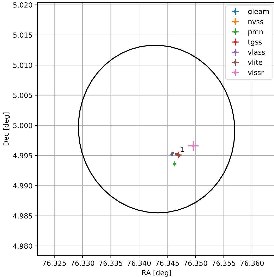
4FGL J0505.3+0459
