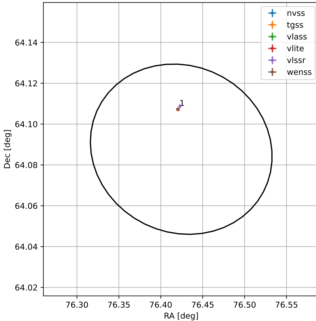
4FGL J0505.6+6405
