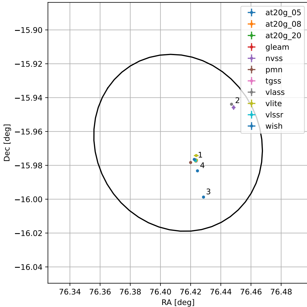
4FGL J0505.6-1558
