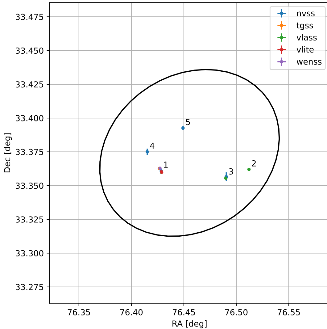
4FGL J0505.8+3322
