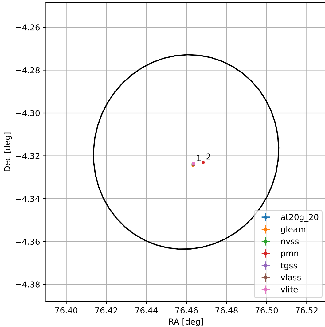
4FGL J0505.8-0419
