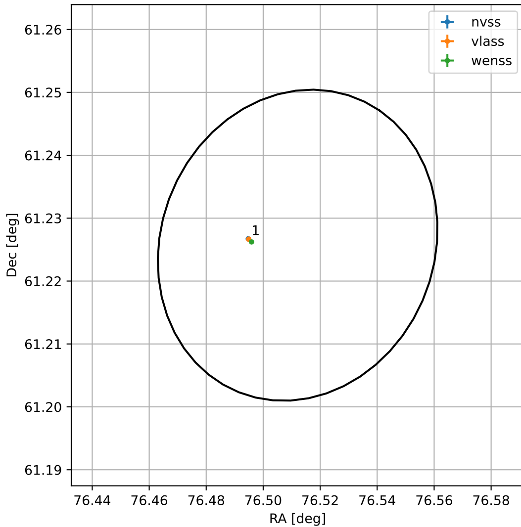
4FGL J0506.0+6113
