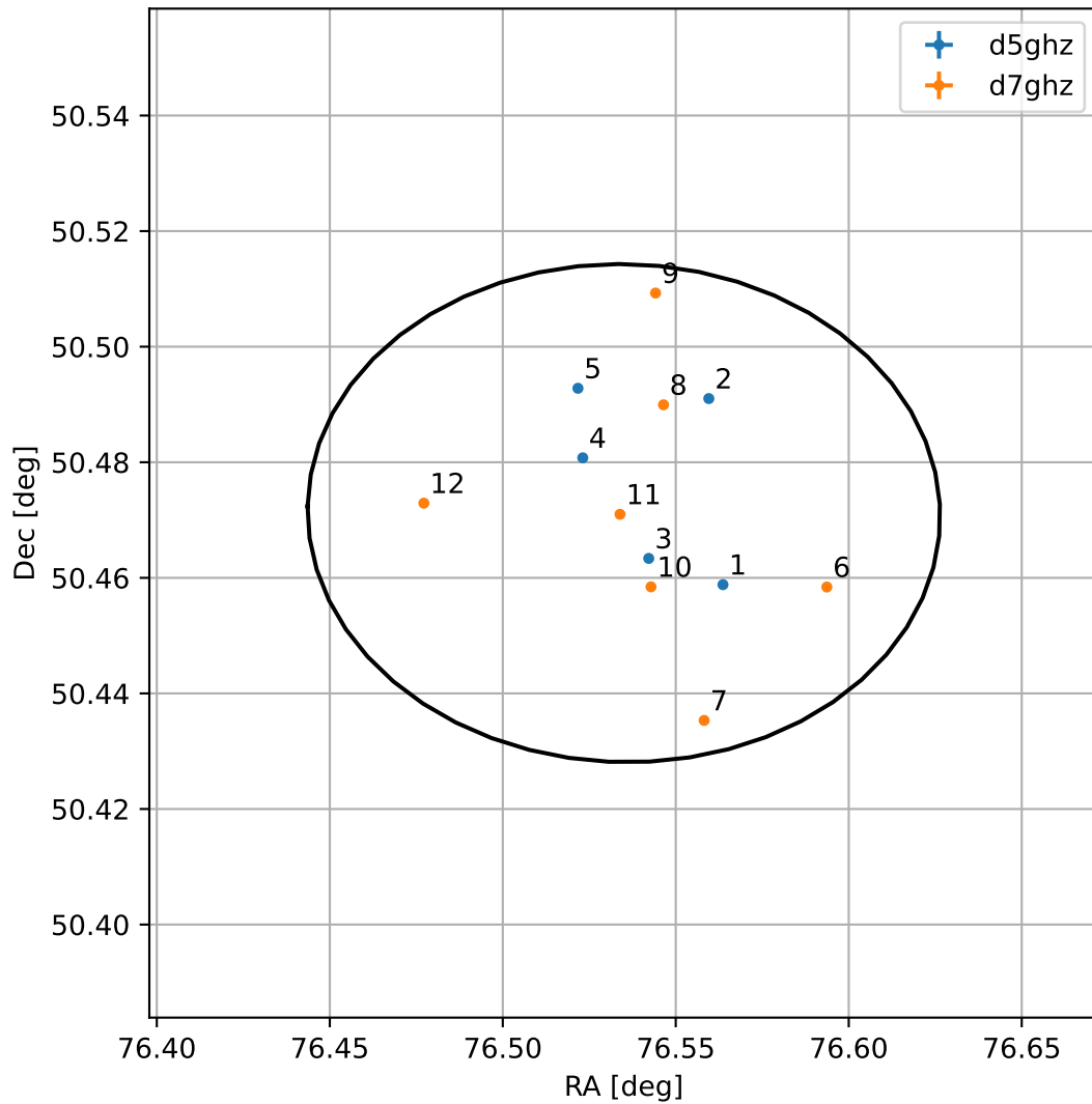
4FGL J0506.1+5028
