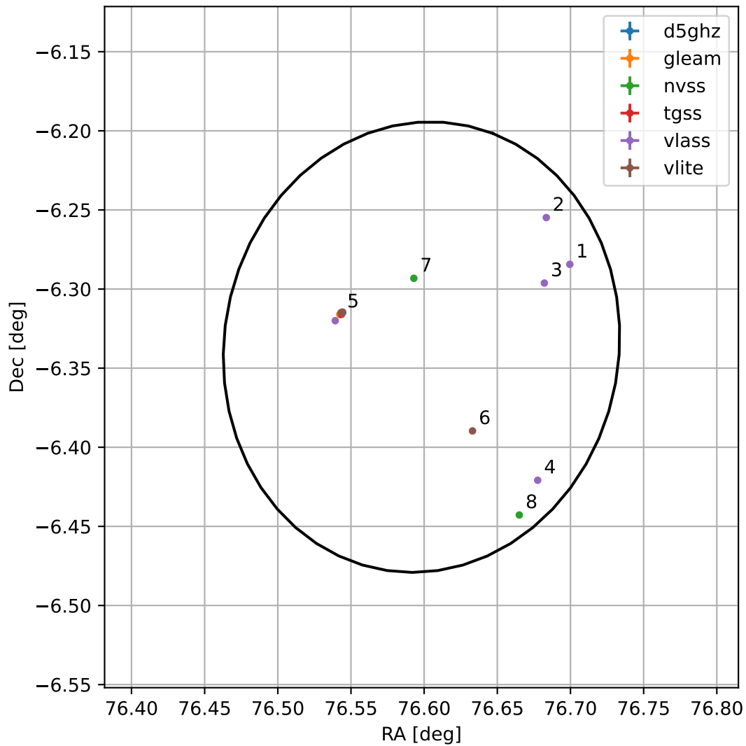
4FGL J0506.3-0620
