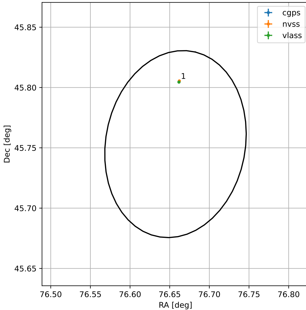
4FGL J0506.6+4545
