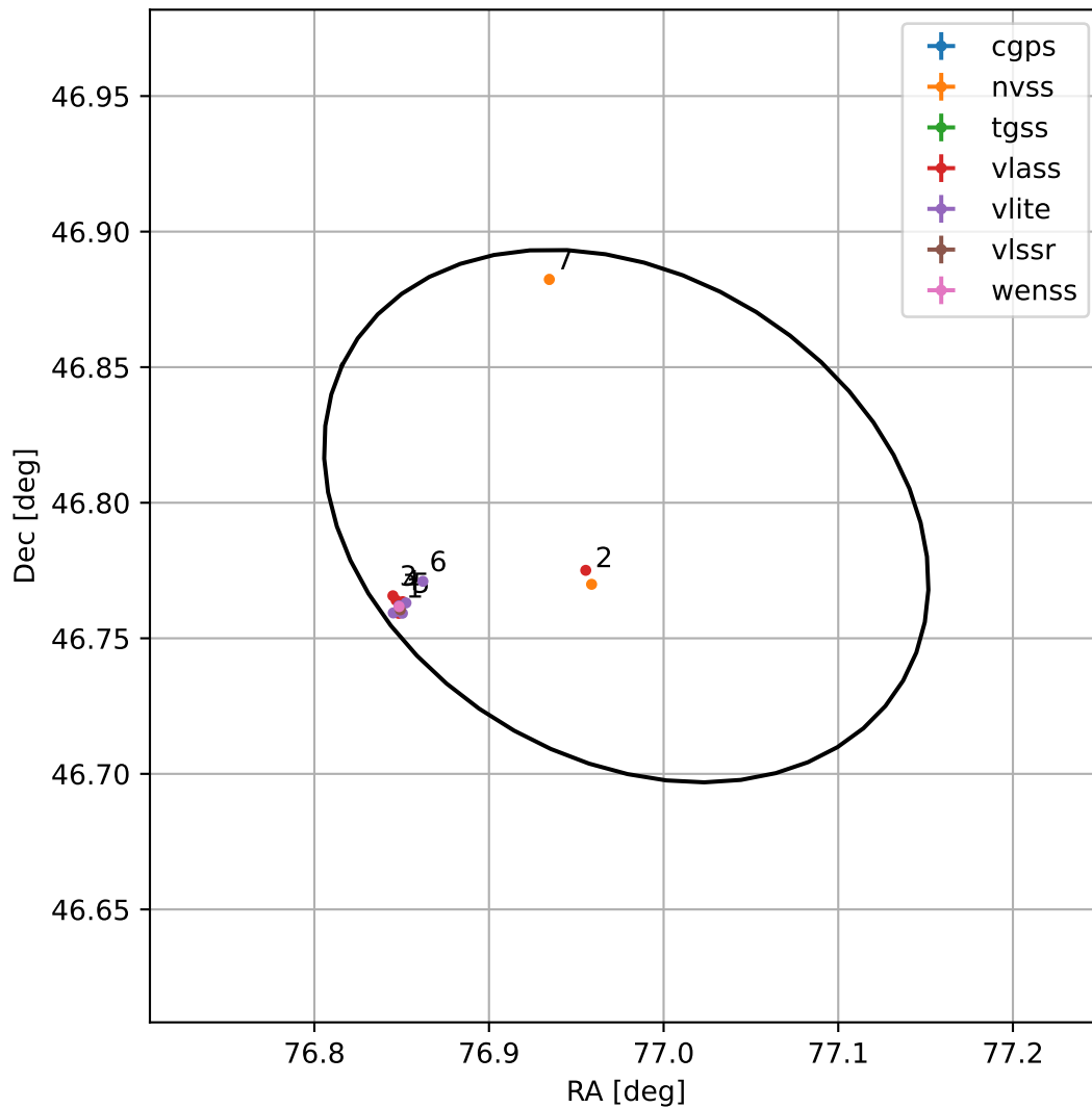
4FGL J0507.9+4647
