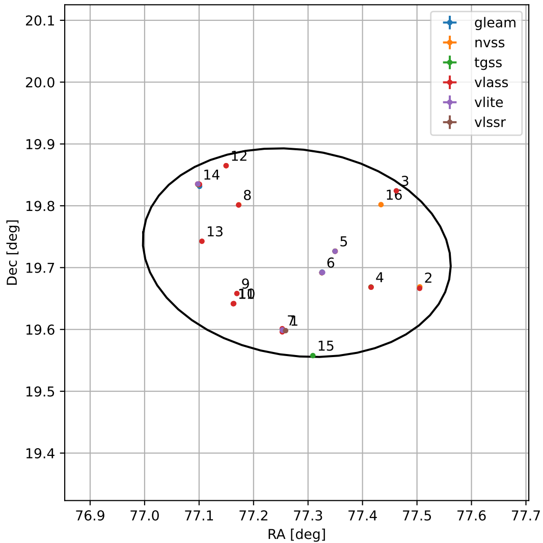
4FGL J0509.1+1943
