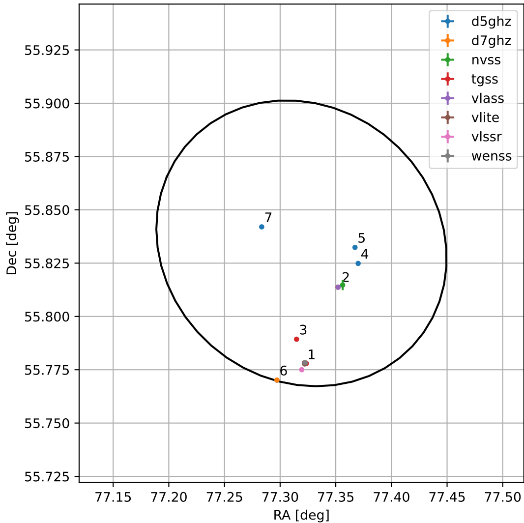
4FGL J0509.2+5550
