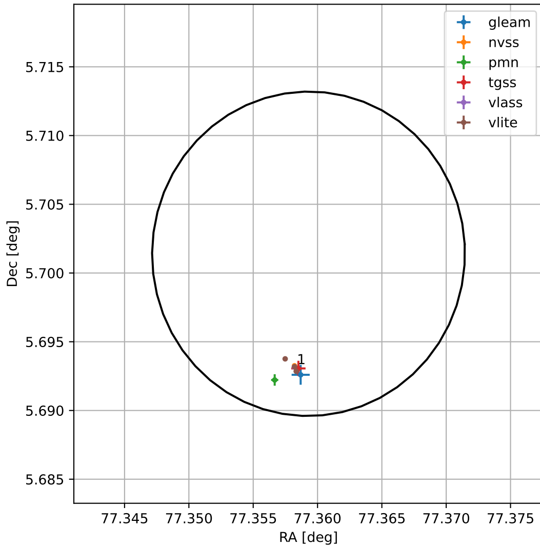
4FGL J0509.4+0542
