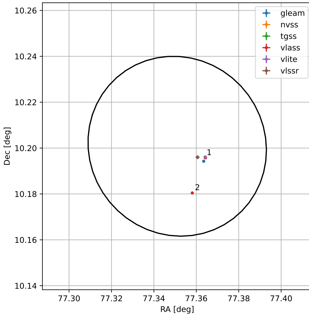
4FGL J0509.4+1012
