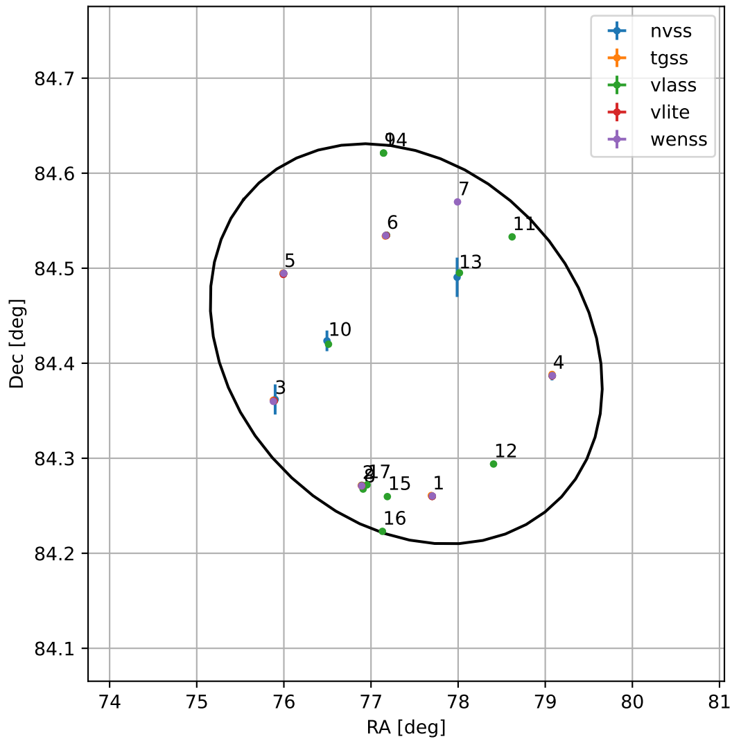
4FGL J0509.6+8425
