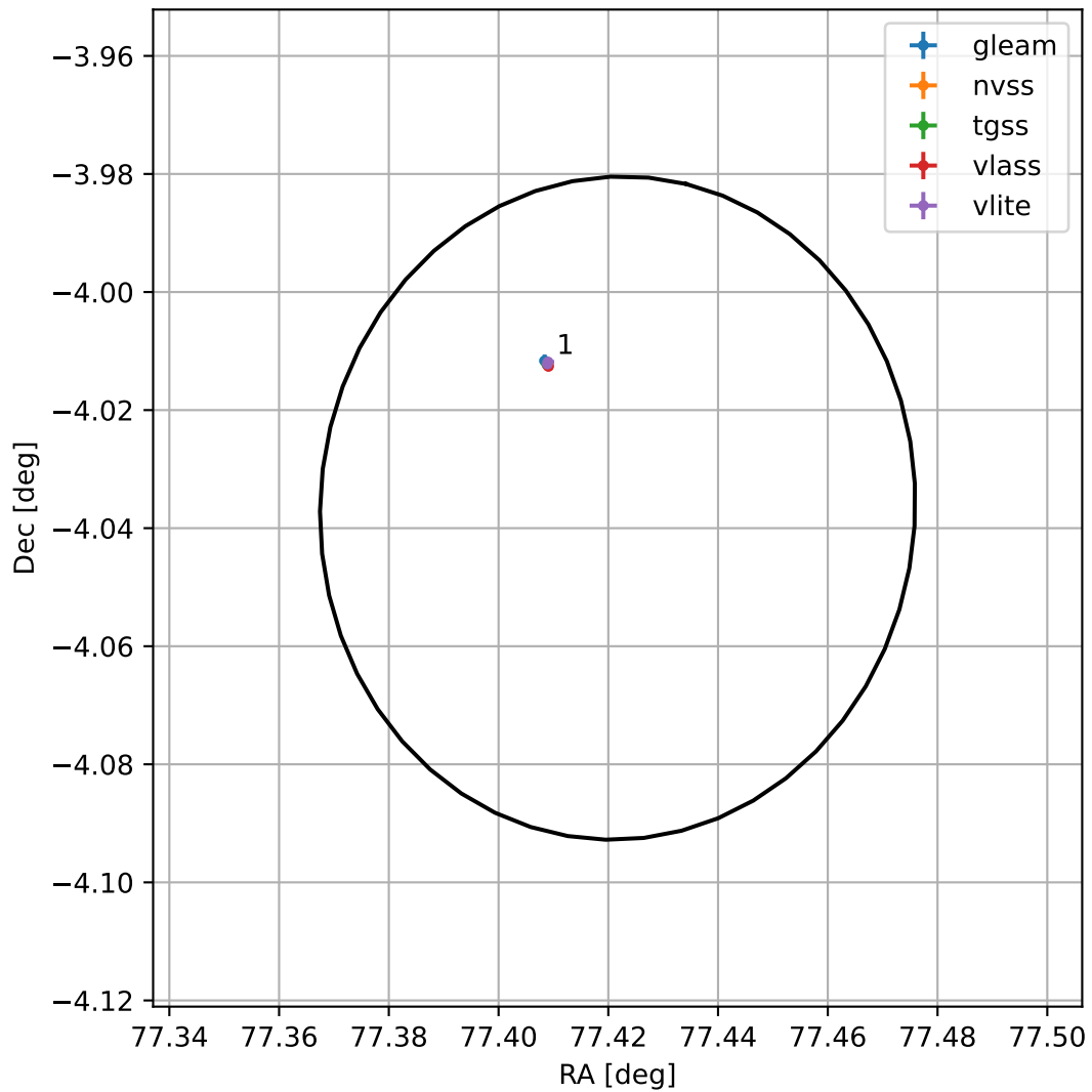
4FGL J0509.6-0402
