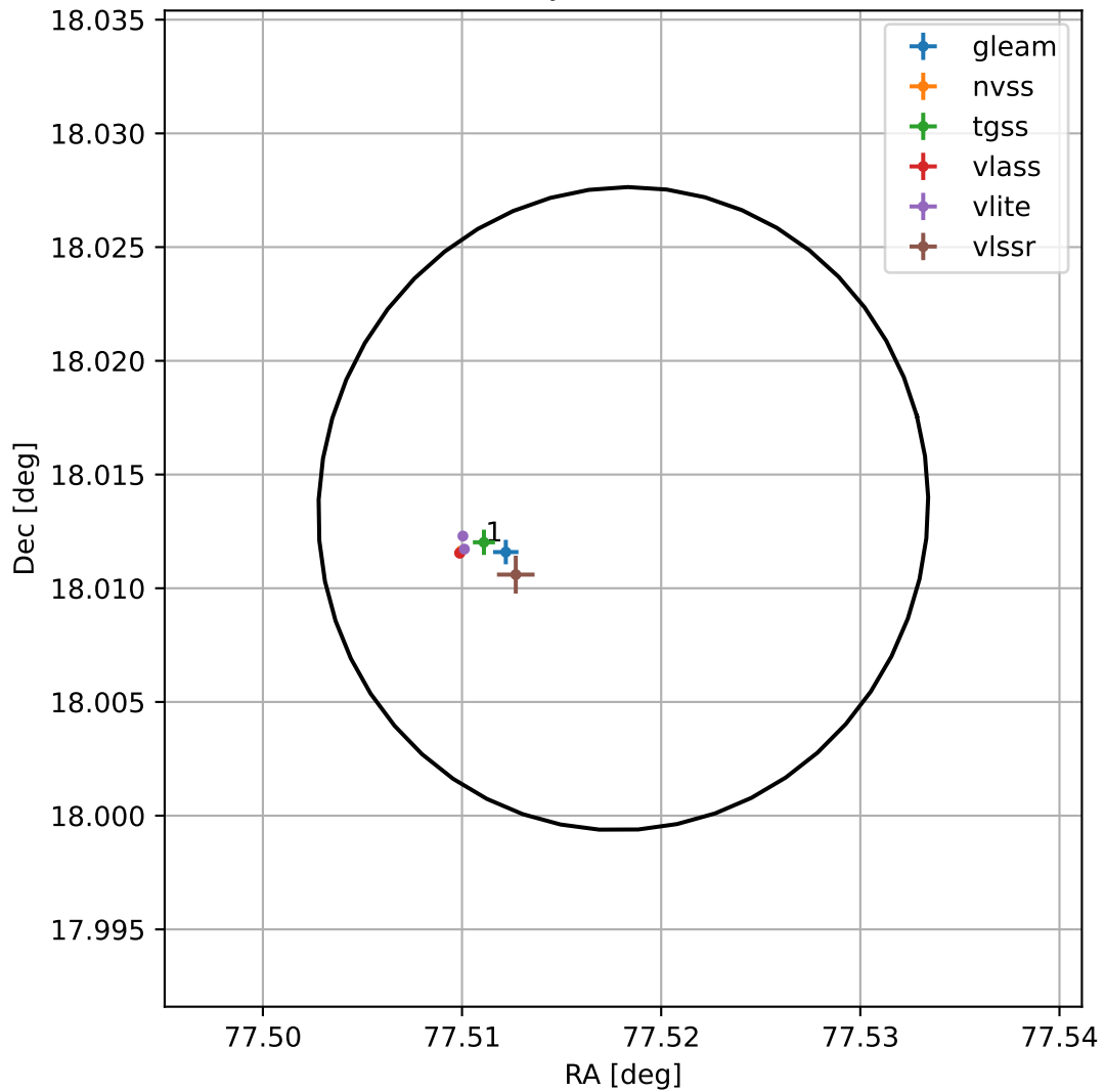
4FGL J0510.0+1800
