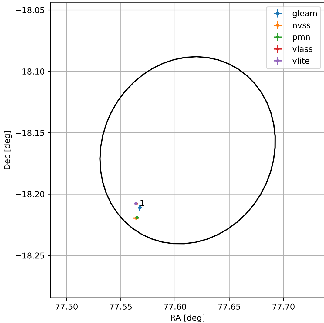
4FGL J0510.4-1809
