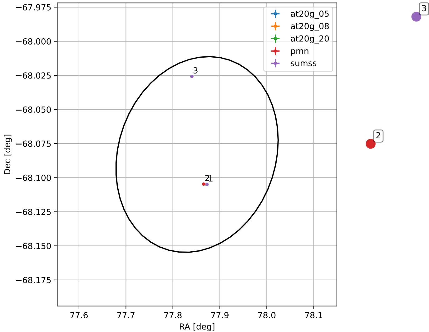
4FGL J0511.4-6804
