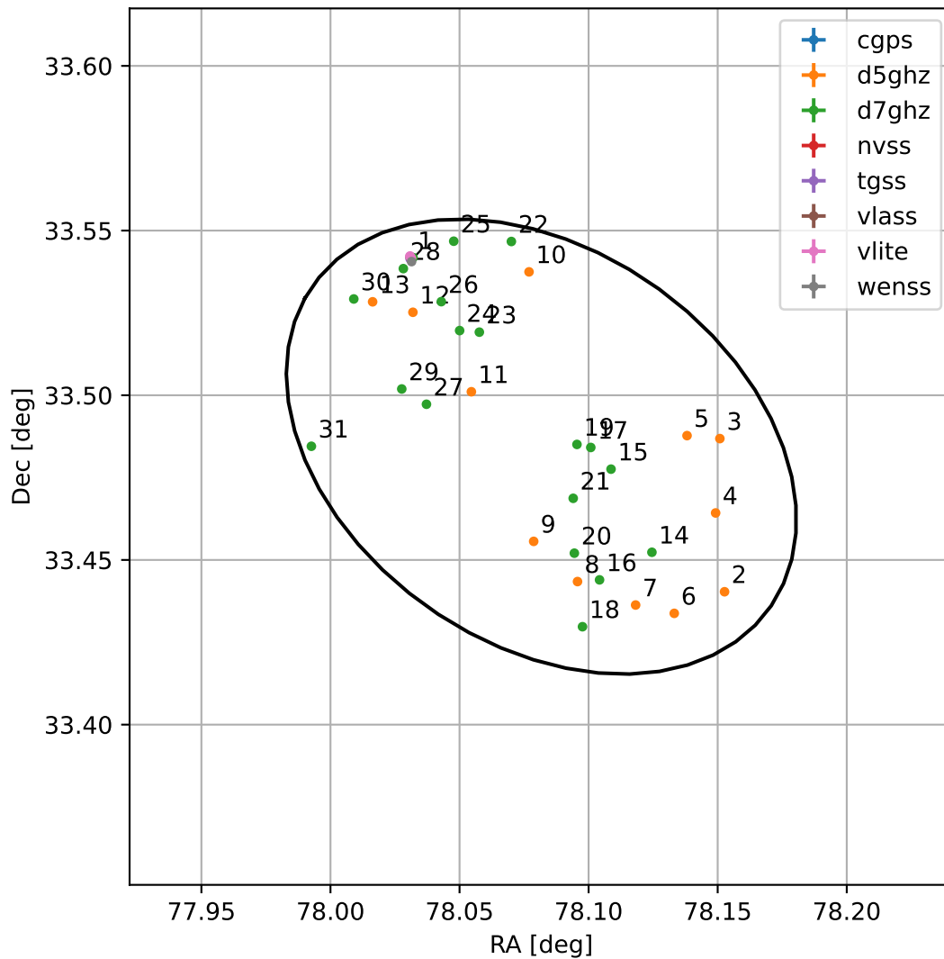
4FGL J0512.3+3329
