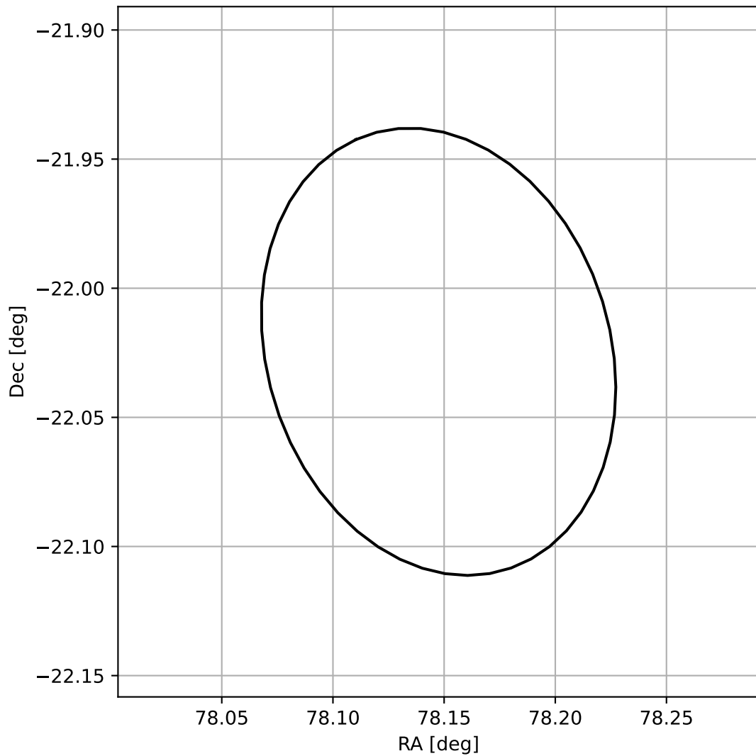
4FGL J0512.5-2201
