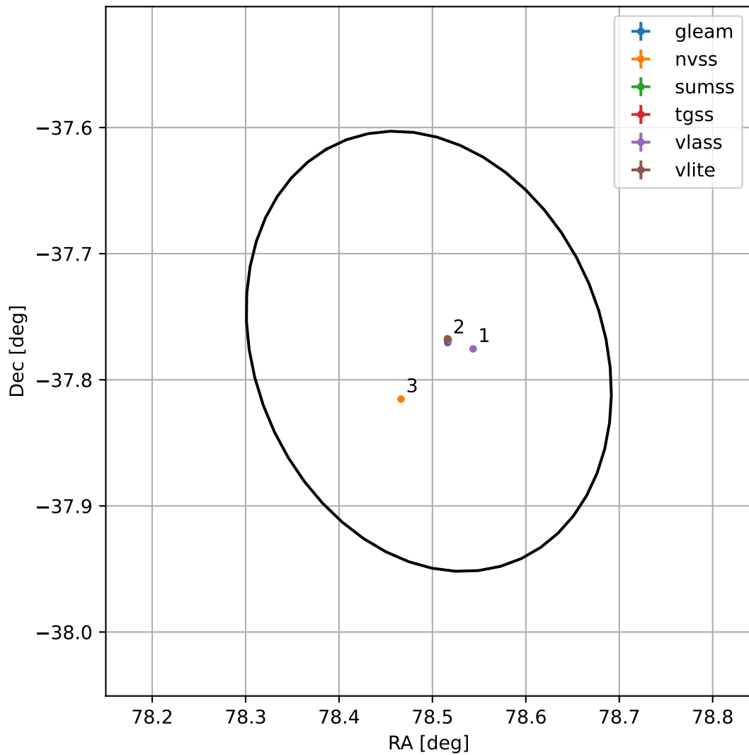
4FGL J0513.9-3746
