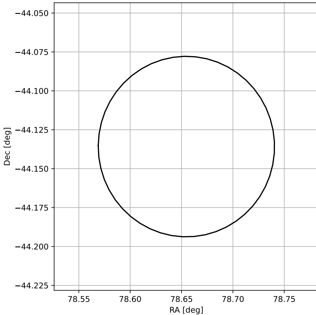
4FGL J0514.6-4408
