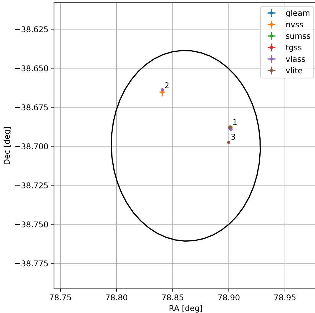
4FGL J0515.4-3841
