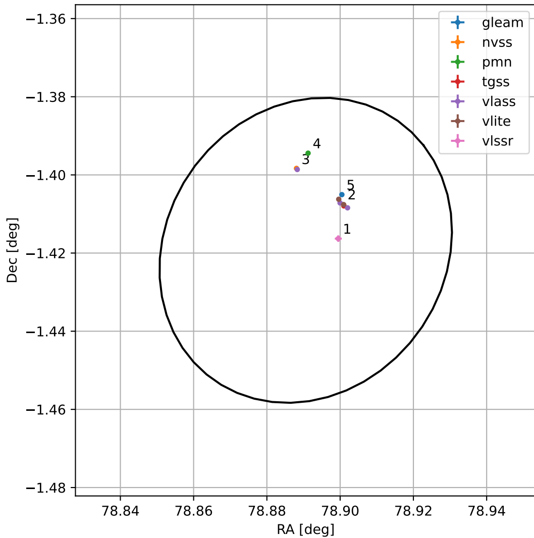
4FGL J0515.5-0125
