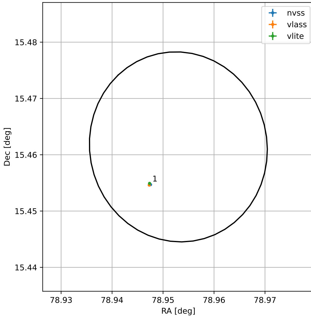
4FGL J0515.8+1527
