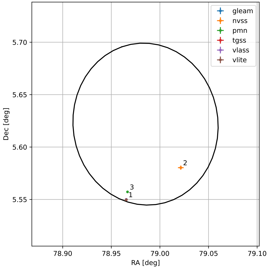
4FGL J0515.9+0537
