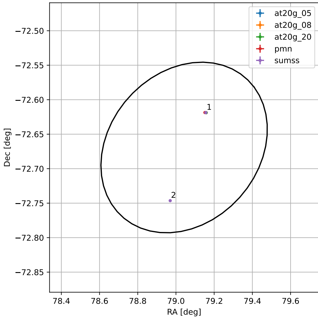
4FGL J0516.1-7240
