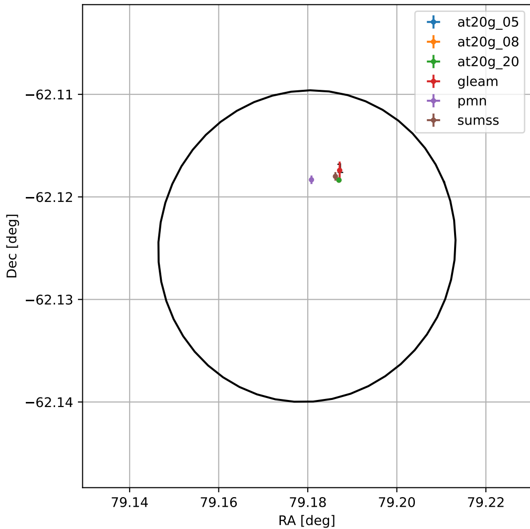
4FGL J0516.7-6207
