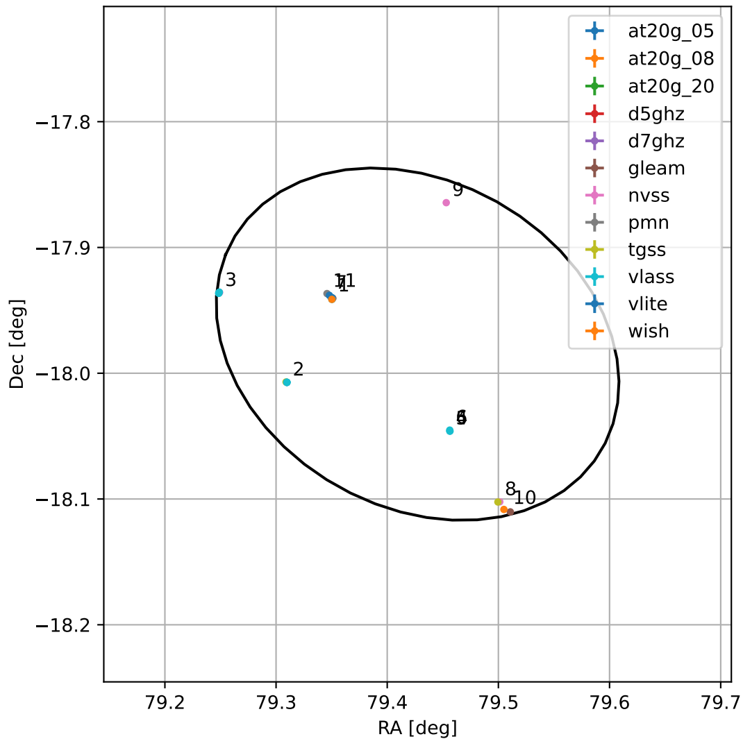
4FGL J0517.7-1758
