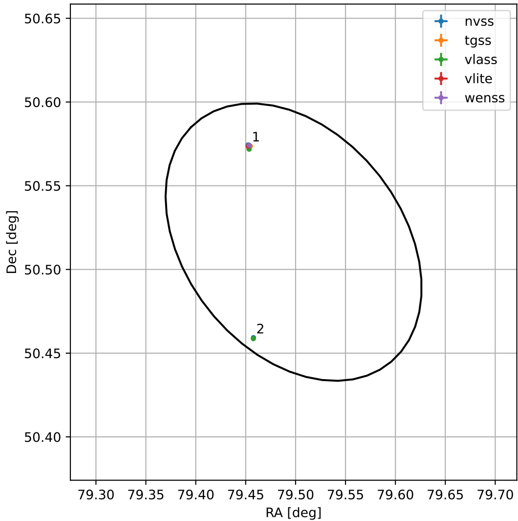
4FGL J0517.9+5030
