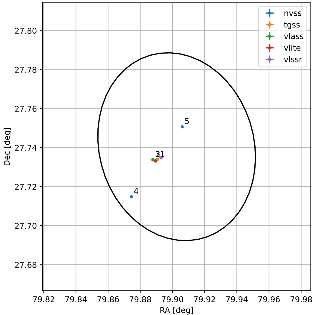
4FGL J0519.6+2744
