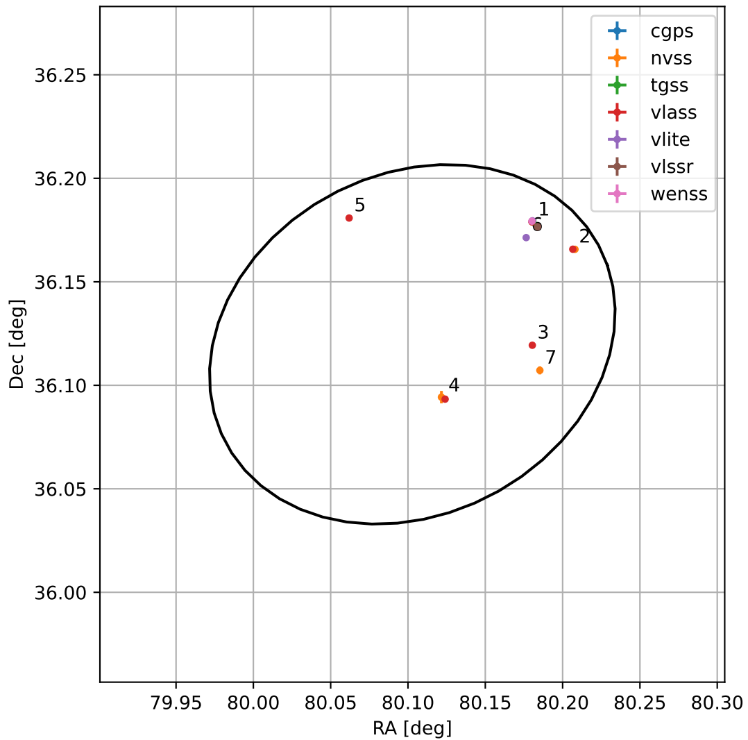
4FGL J0520.4+3607
