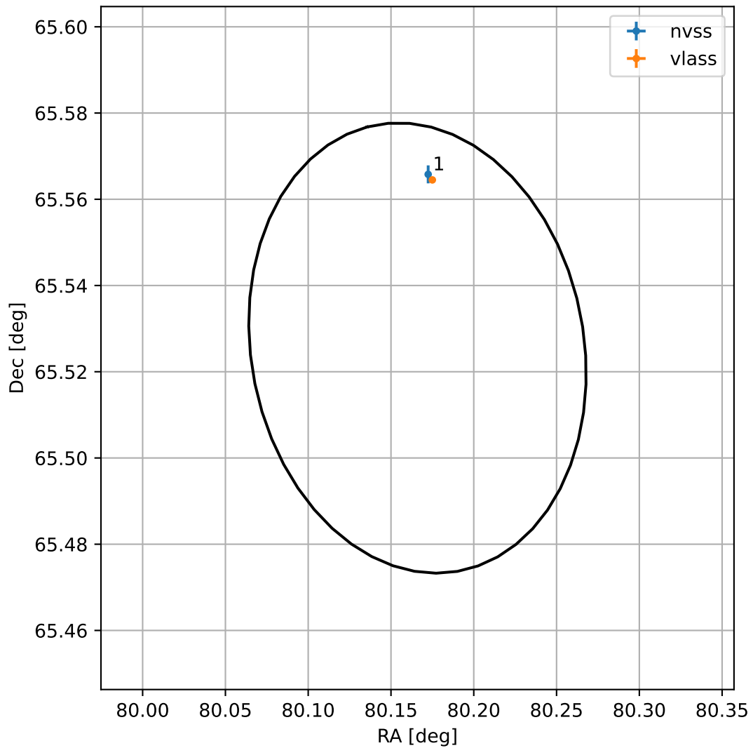
4FGL J0520.6+6531
