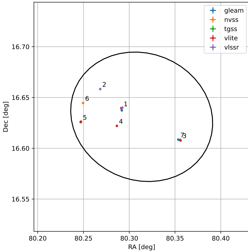
4FGL J0521.2+1637
