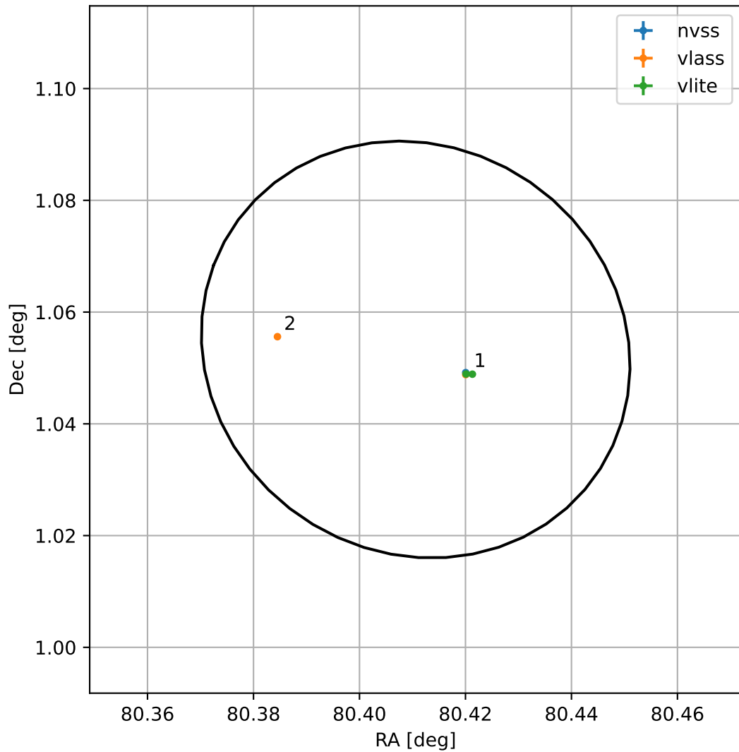
4FGL J0521.6+0103
